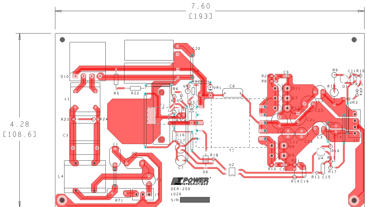
Figure 3 – PCB Layout.
