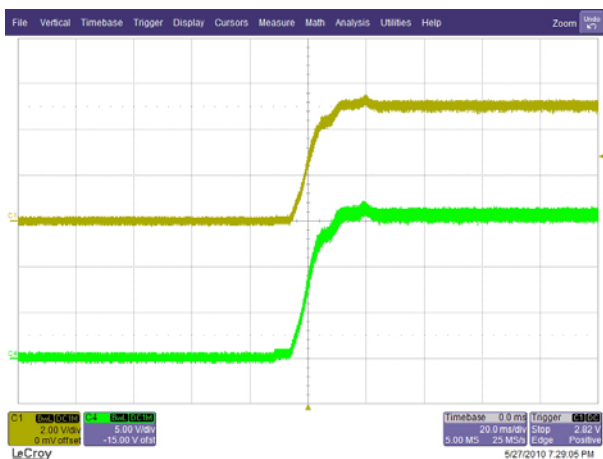
Figure 16 – Start-up Profile, 90 VAC. Upper: V_{5V} , 2 V / div. Lower: V_{16V} , 5 V, 20 ms / div.
