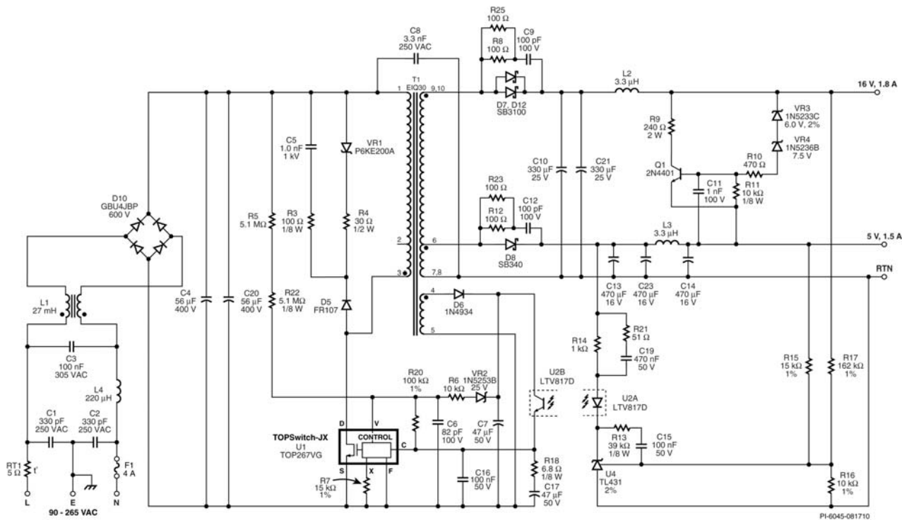
Figure 2 – Schematic.
