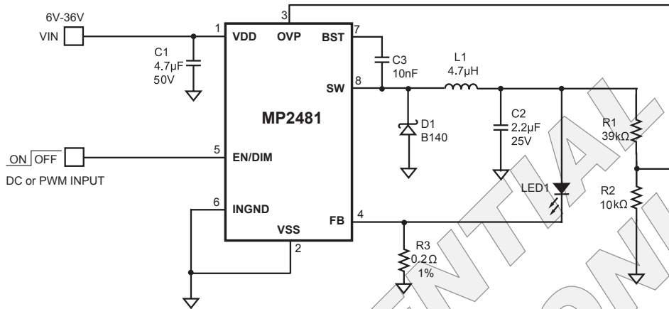
Figure 2—Step-Down White LED Driver Application
