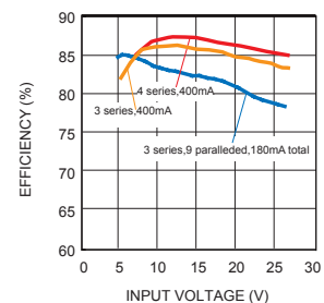
Efficiency vs. Input Voltage Step-up/down Application
