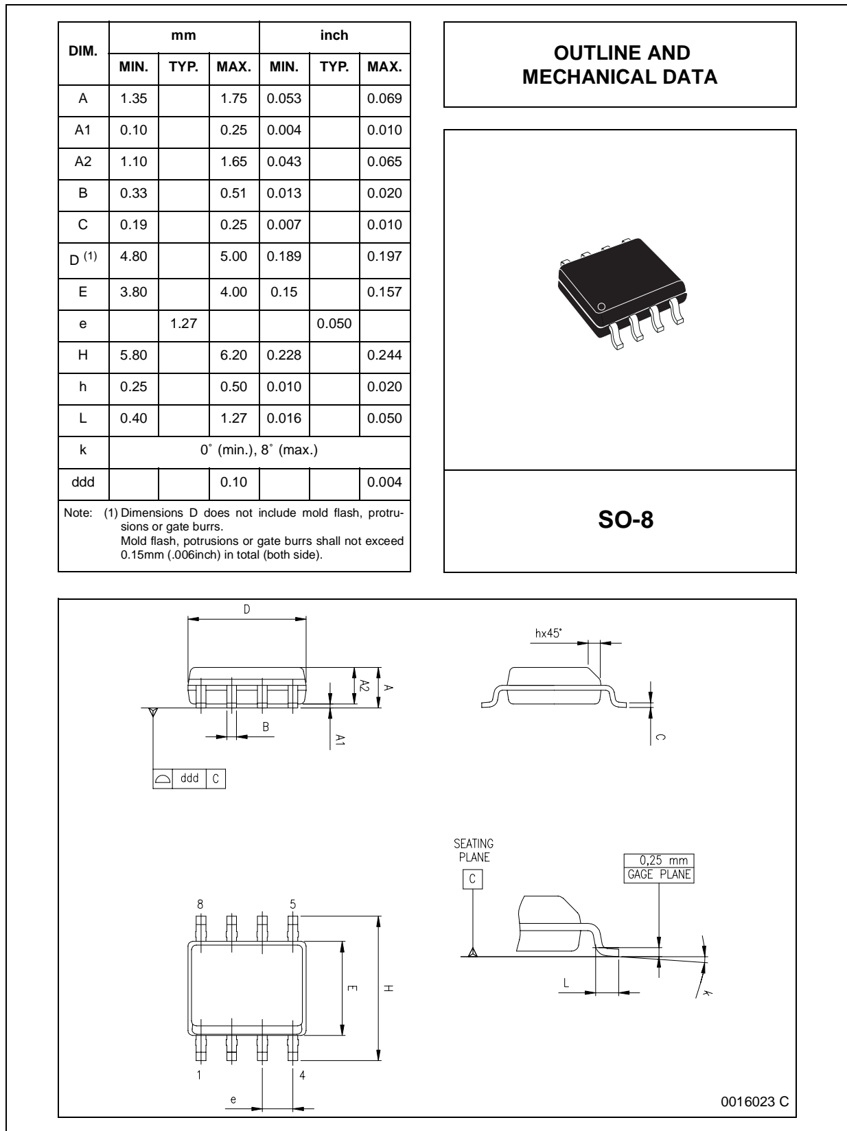
Figure 28. SO-8 Mechanical Data & Package Dimensions
