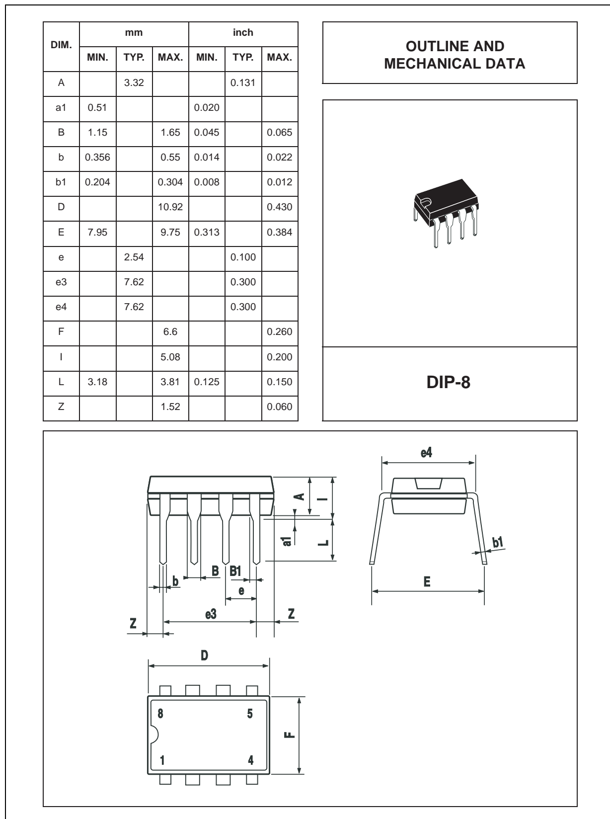
Figure 27. DIP-8 Mechanical Data & Package Dimensions
