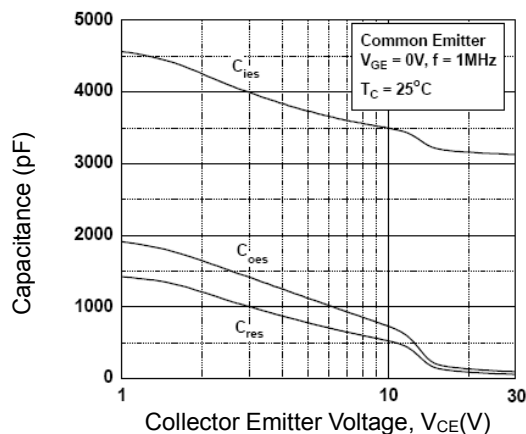
Figure 6. Capacitance Characteristics
