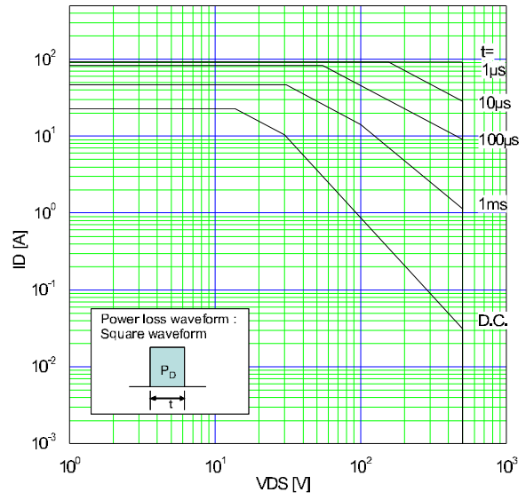
Safe Operating Area I_c = f(V_{DS}): \text{Duty}=0(\text{Single pulse}), T_c=25^\circ\text{C}
