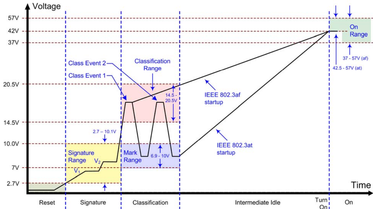
Figure 1 - 802.3at Typical Power-On Waveform
