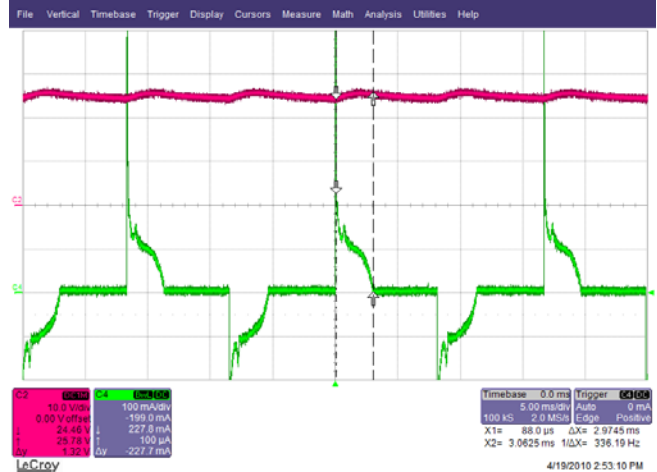
Figure 31 – 115 VAC, 65° Phase. Upper: V_{OUT} , 10 V / div. Lower: I_{IN} , 0.1 A / div., 5 ms / div.
