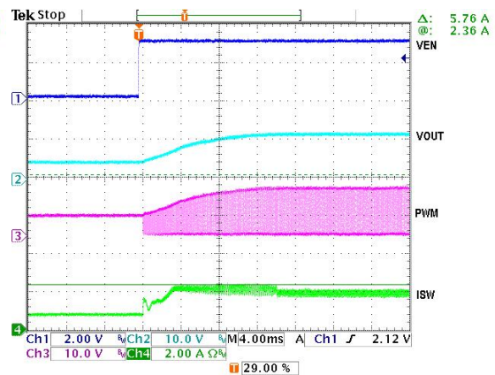
Enable-ON Wave (V CC =5V, V OUT =12V, Load=0.7A, SS=0.1uF)
