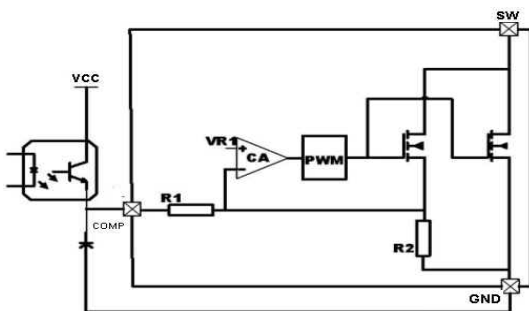
Fig 2 Feedback circuit
