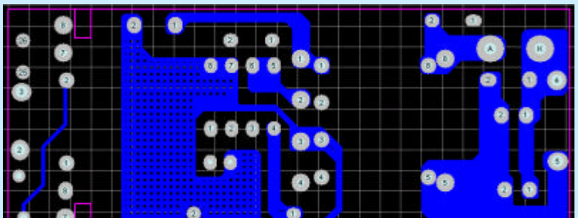
BOTTOM层
