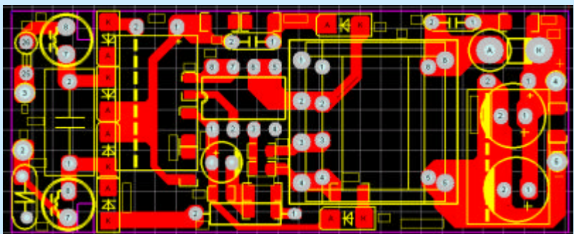
BOTTOM层
