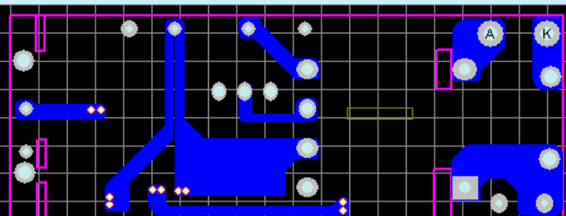
BOTTOM层
