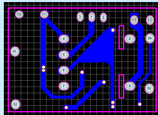
BOTTOM层
