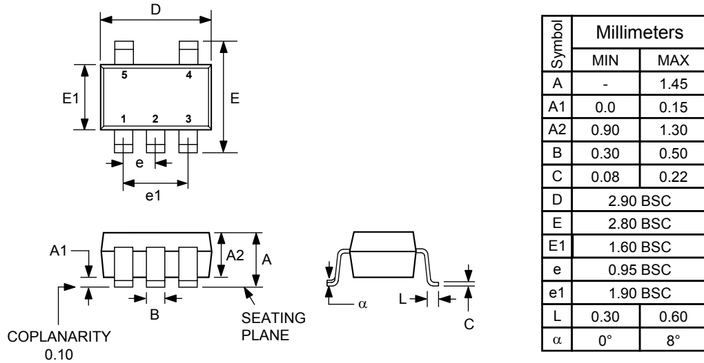
Figure 10.1: Physical dimensions, 5-lead SOT-23 package
