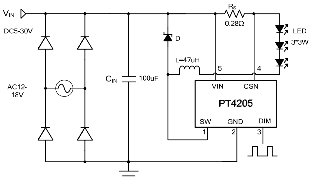
Fig 2: 3X3W application
