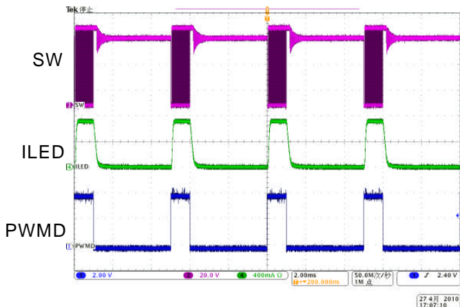
11. PWM Dimming use PWM_D pin
