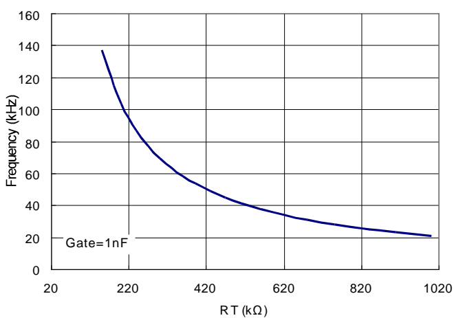
5. RT Resistor vs Switching Frequency
