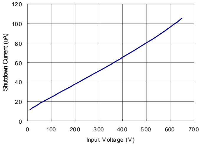
1. Input Voltage vs Shutdown Current
