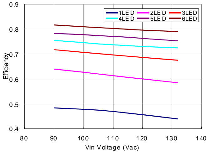
7. Input Voltage vs Efficiency
