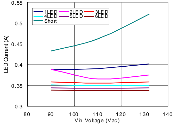
8. Input Voltage vs LED Current
