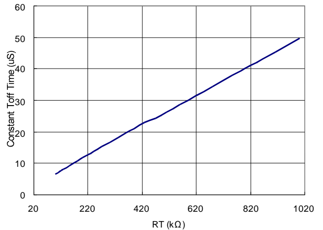
6. RT vs Constant Toff Time
