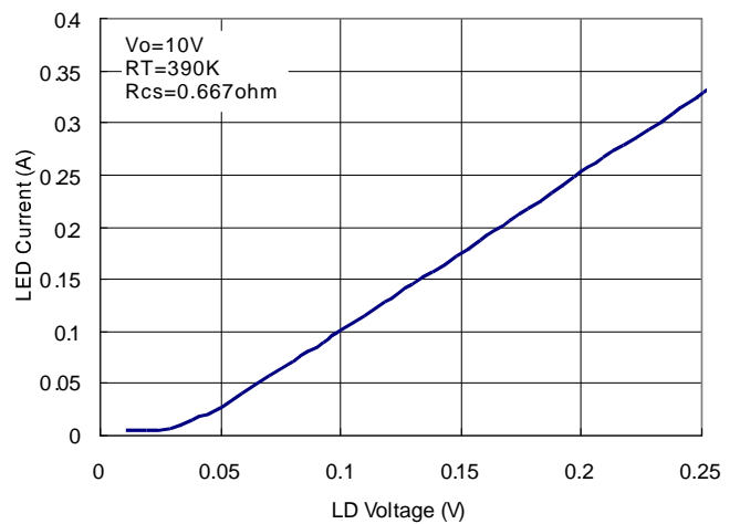
4. LD Voltage vs Output LED Current
