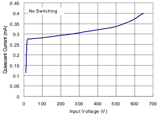
2. Input Voltage vs Supply Current
