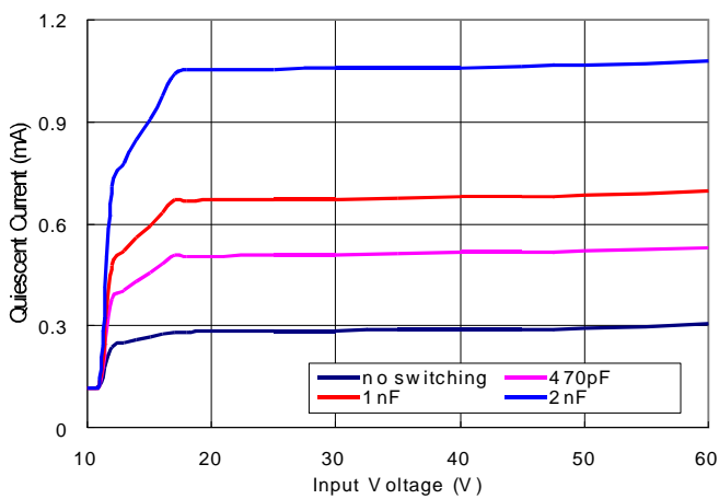
3. Input Voltage vs Quiescent Current
