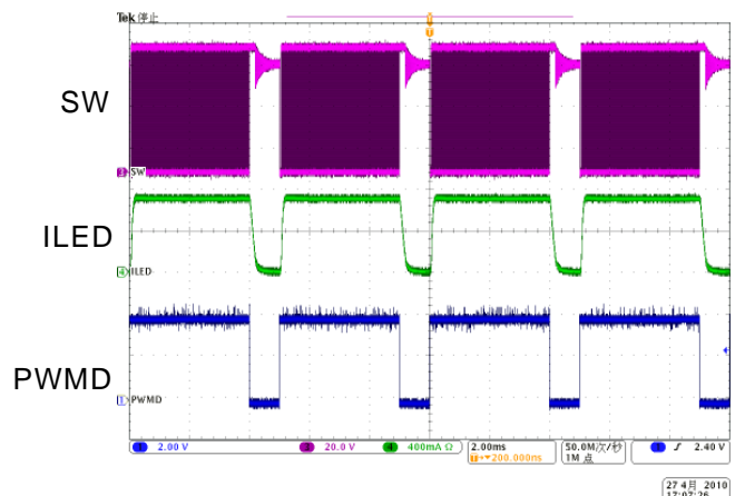
12. PWM Dimming use PWM_D pin
