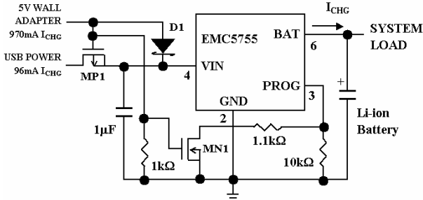
USB/Wall Adapter Power Li-ion Charger
