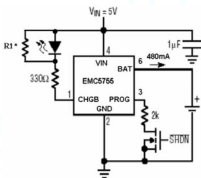
Turn off the LED after Charge is Terminated
