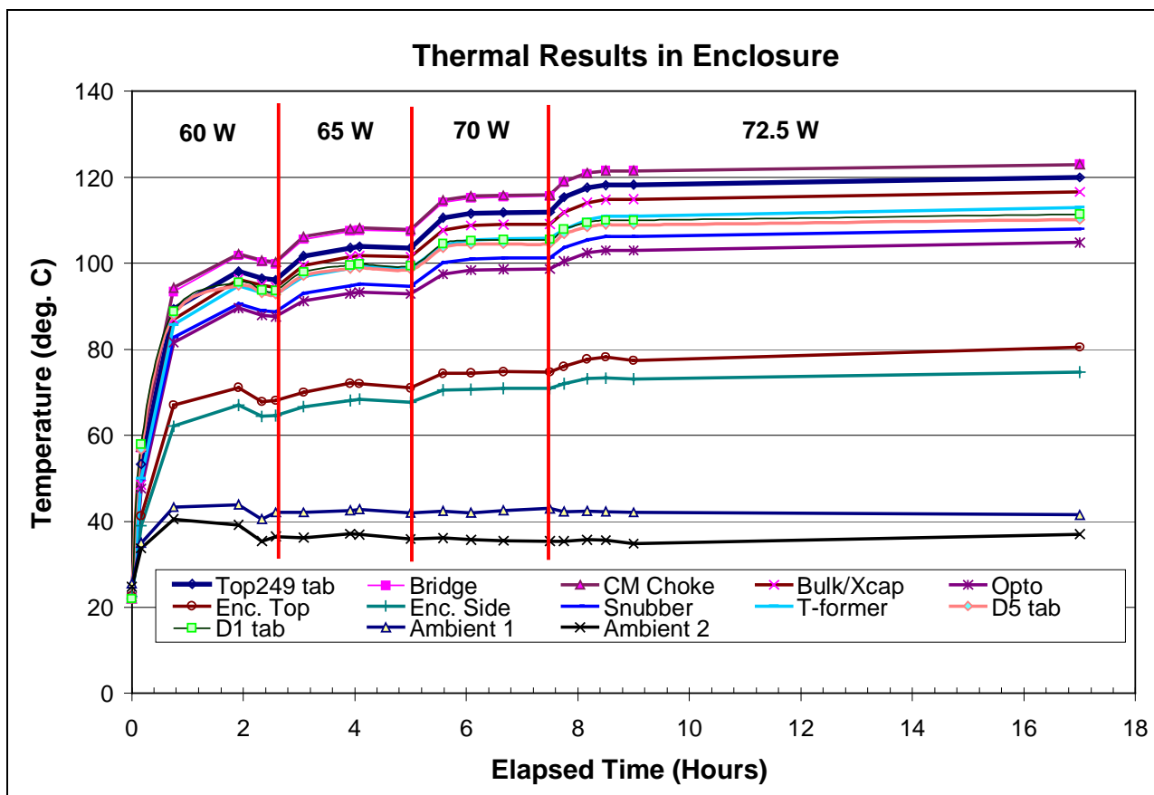
Figure 13 - Thermal results in enclosure at elevated ambient with 60, 65, 70, and 72.5 Watt loads – 90 V AC
