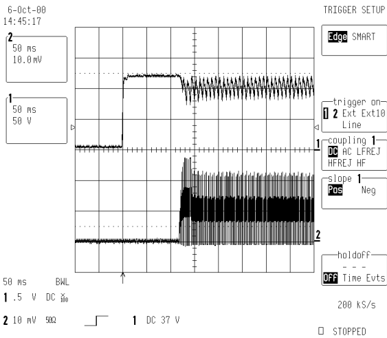
Figure 25 - Start-up, 5.25 \Omega load, 85 V_{AC} V_{C7} & I_{DRAIN} (50 V & 1A/div, 50ms/div)
