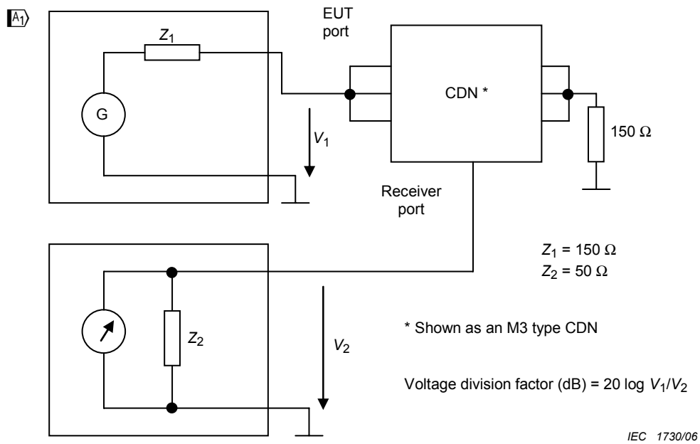
Figure B.2 – Calibration set-up for determining CDN voltage division factor
