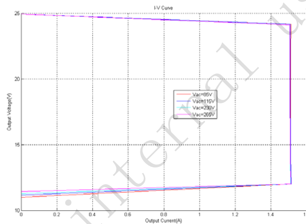
Fig. 4 CC/CV Characteristics
