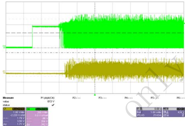
Fig. 13 Start, Vds waveform@264 Vac/50Hz, full load
