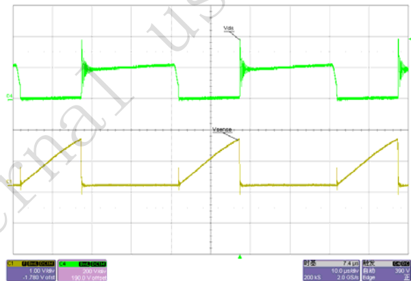
Fig. 15 Normal, Vds&Ids waveform@90 Vac/60Hz, full load
