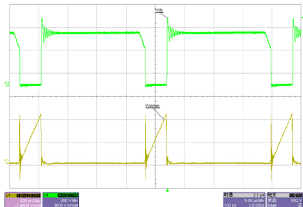
Fig. 17 Normal, Vds&Ids waveform@264 Vac/60Hz, full load
