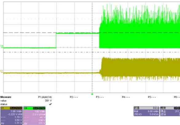
Fig. 12 Start, Vds waveform@90 Vac/60Hz, full load
