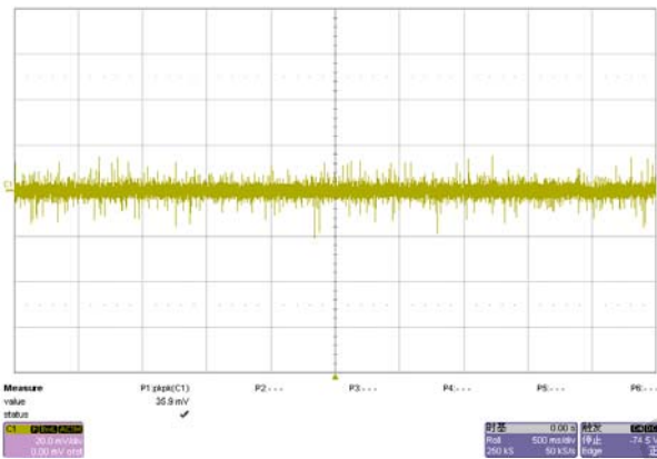
Fig. 7 Measured ripple& noise waveform @264Vac/50Hz, no load
