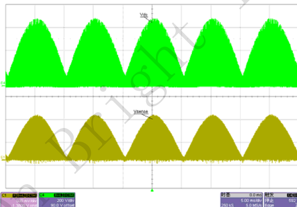
Fig. 16 Normal, Vds&Ids waveform@264 Vac/60Hz, full load
