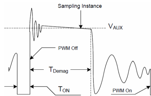
Fig.2. Auxiliary voltage waveform
