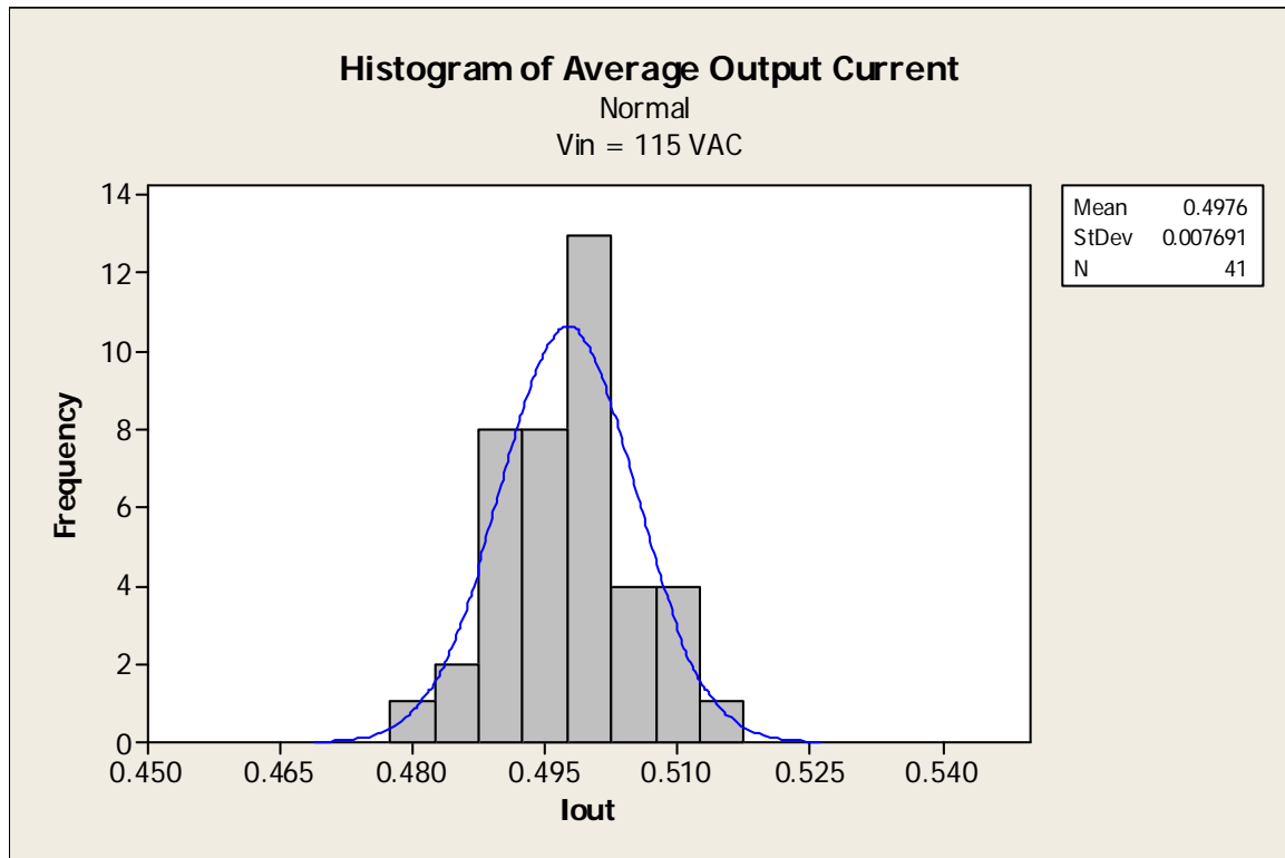
Figure 40 – Production Variation of I_{OUT}
