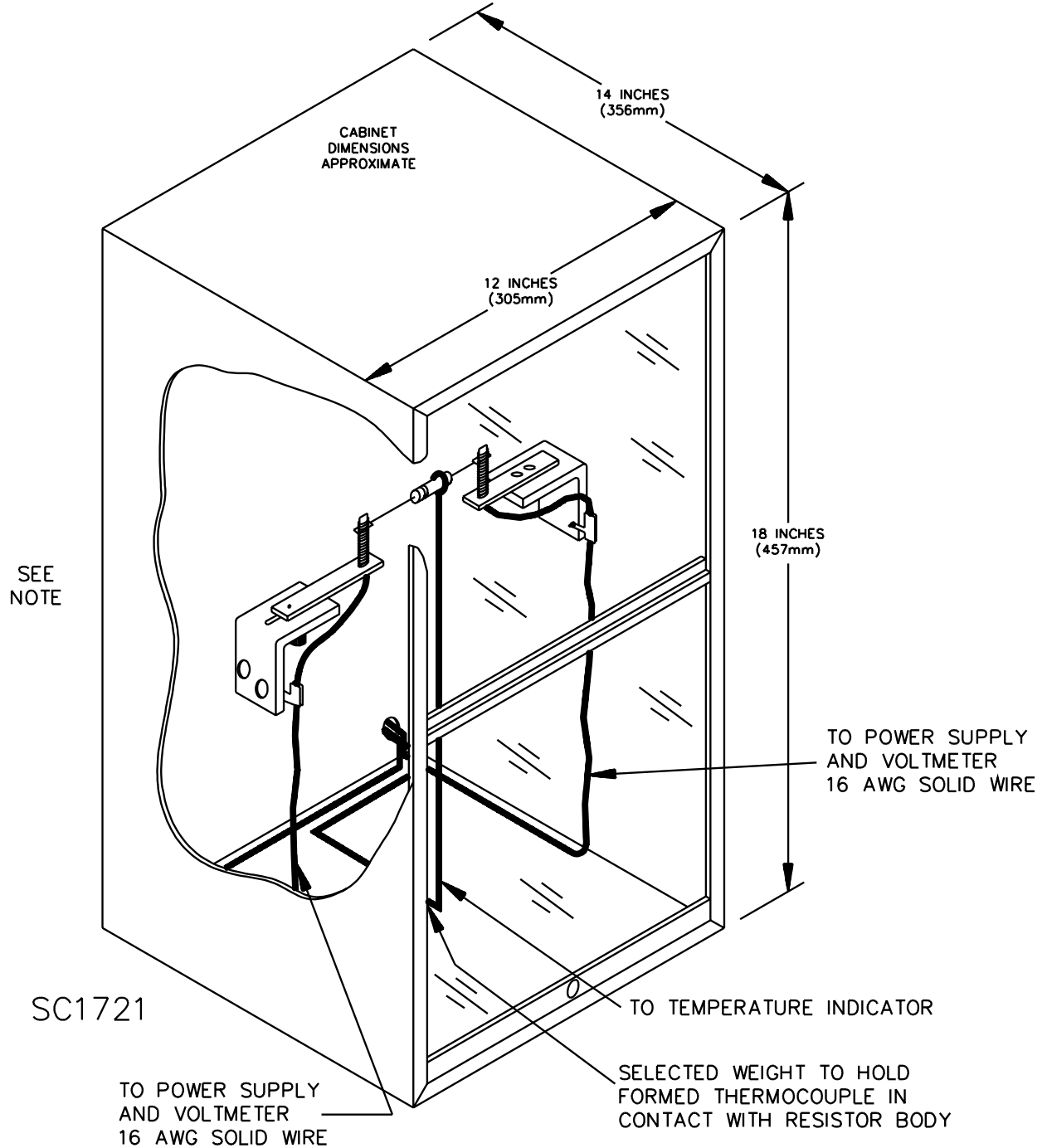
Figure 21.1 Overload test equipment and circuit
