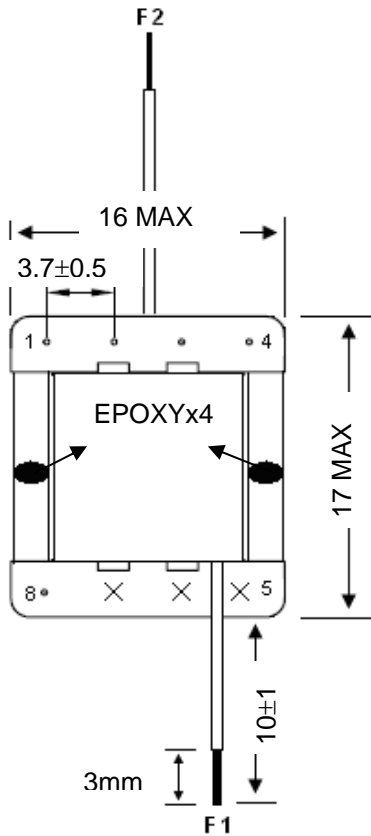
<BOTTOM VIEW>
