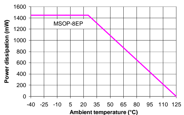
Figure 5. Derating Curve
