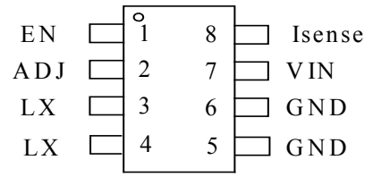
T6322A-ADG SOP-8
