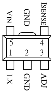
T6322A-EXG SOT-89-5
