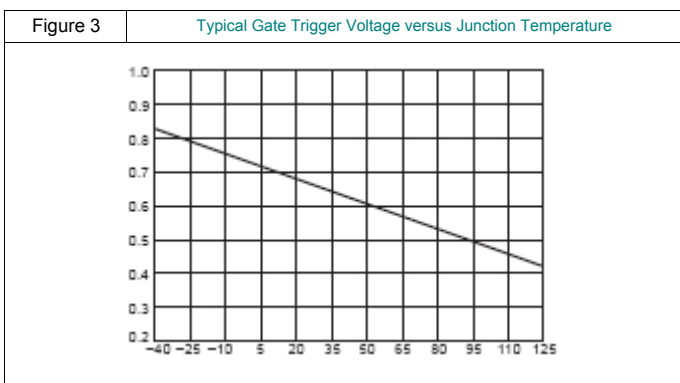
V_{GT} , GATE TRIGGER VOLTAGE(V); T_J , JUNCTION TEMPERATURE (°C)
