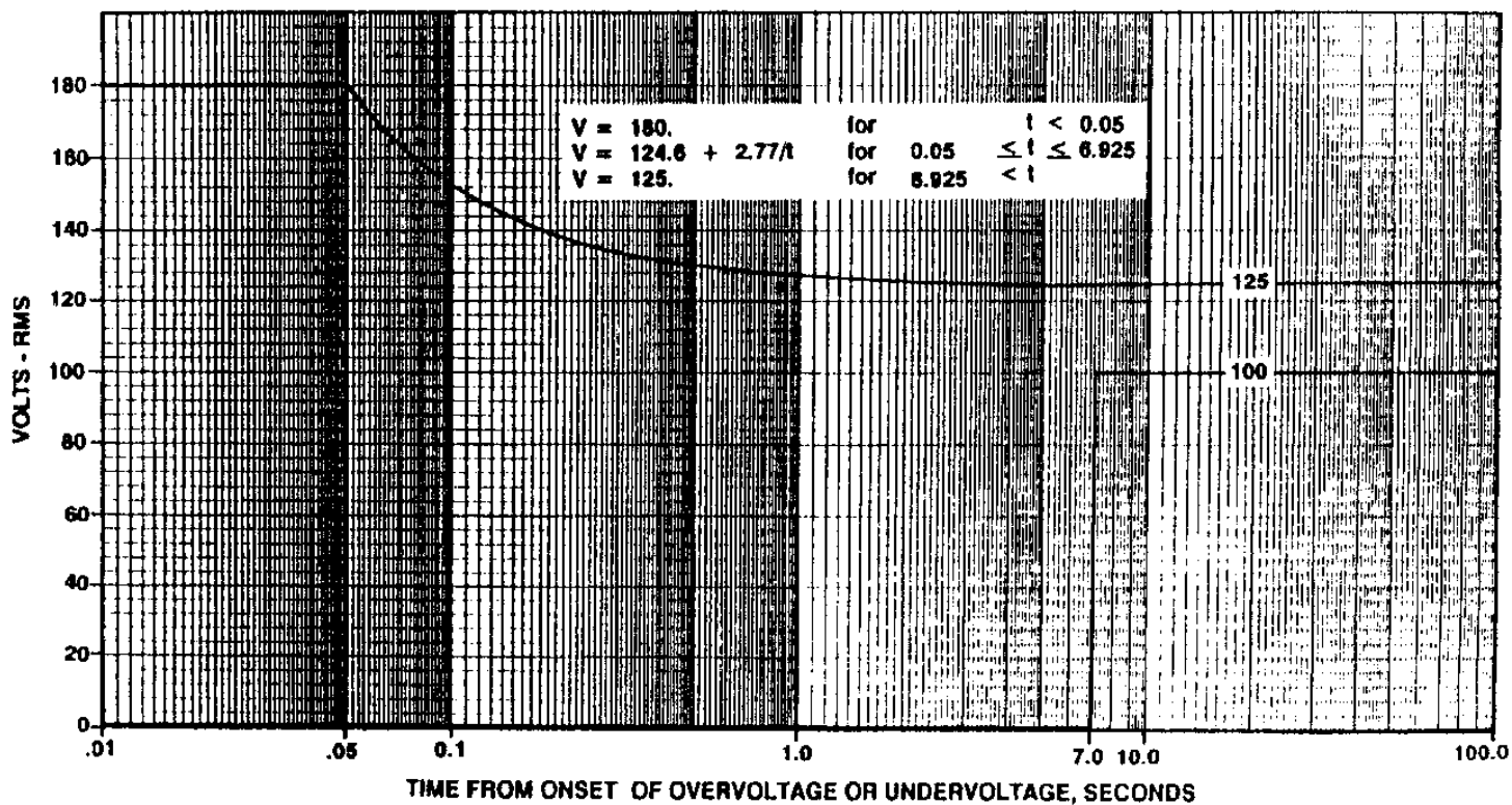
FIGURE 6. Limits for AC overvoltage or undervoltage.
