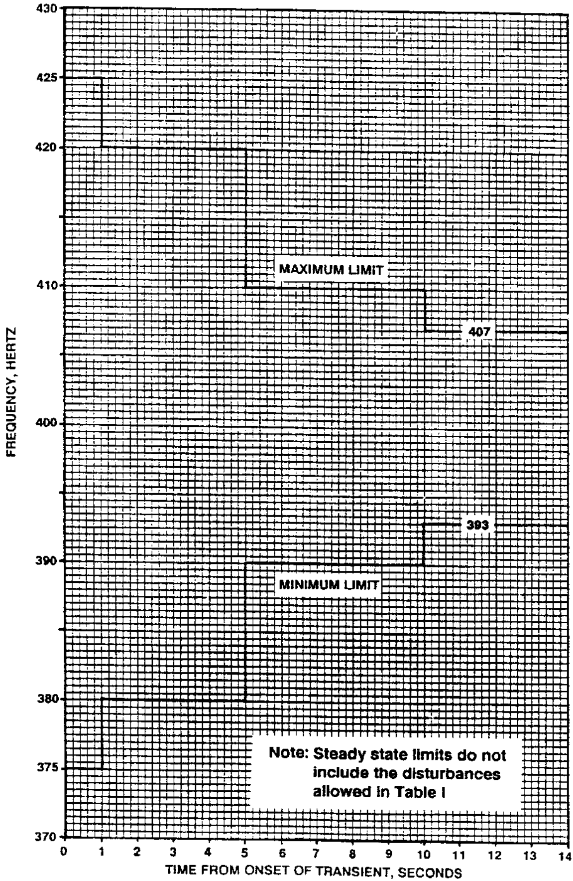
FIGURE 5. Envelope of normal AC frequency transient.
