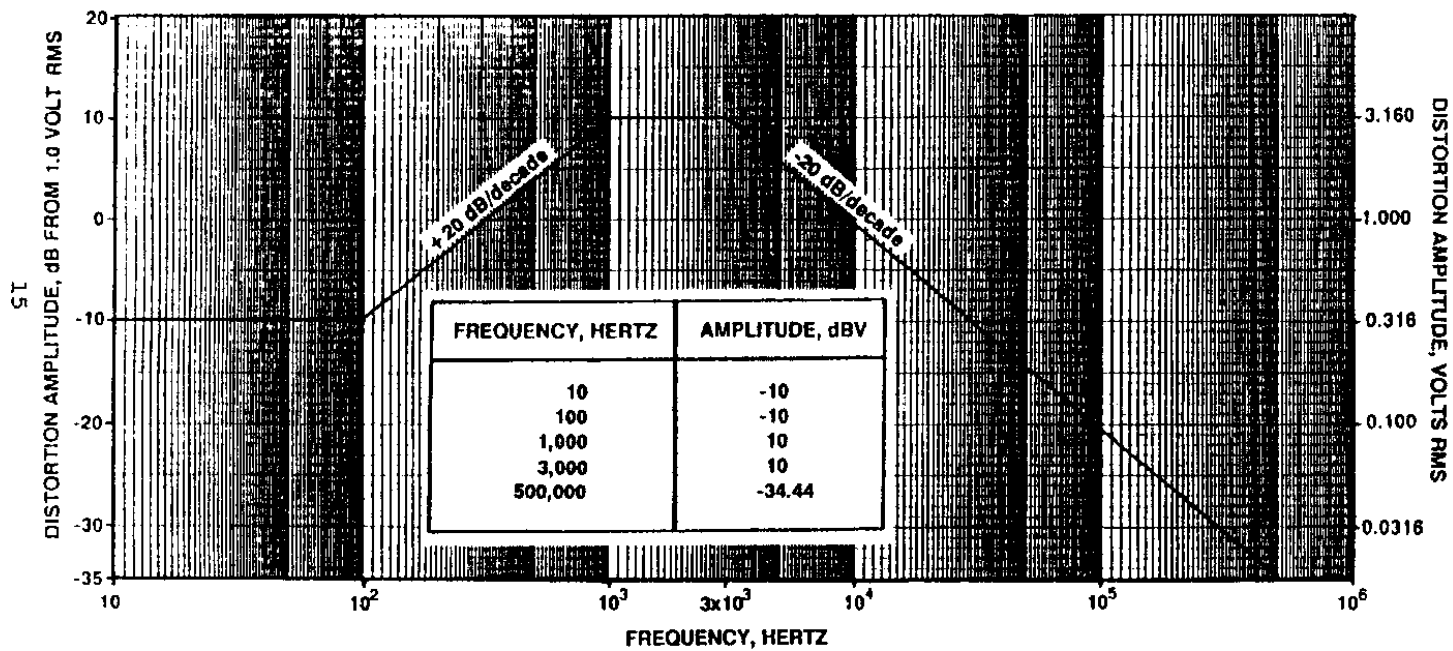
FIGURE 3. Maximum distortion spectrum of AC voltage.
