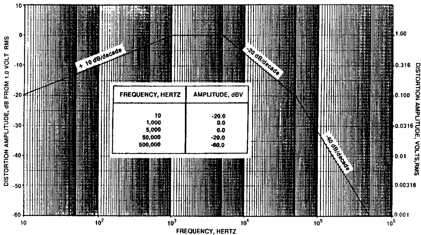
FIGURE 8. Maximum distortion spectrum for 28 volts DC system.
