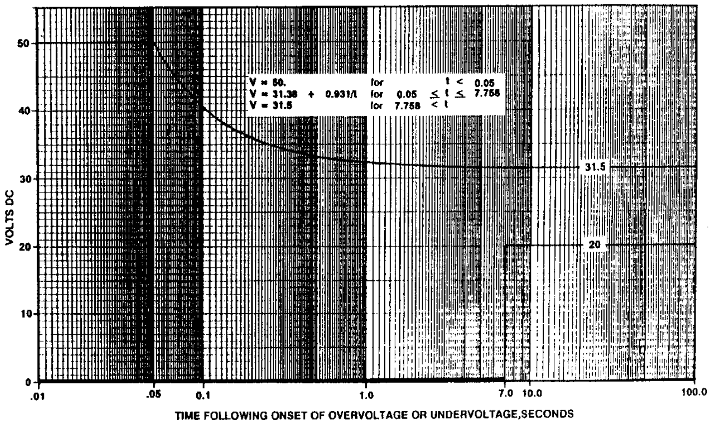
FIGURE 11. Limits for DC overvoltage or undervoltage for 28 volts DC system.
