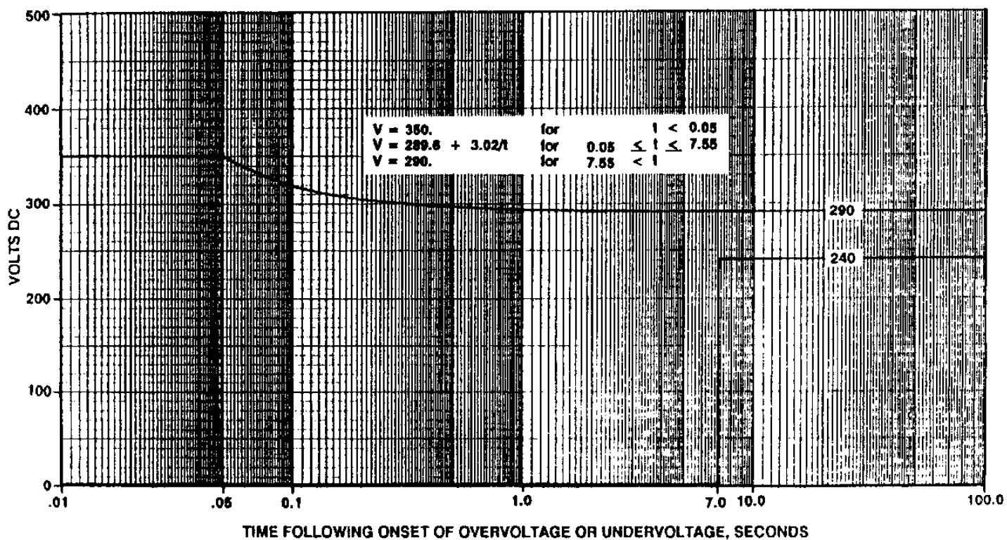
FIGURE 12. Limits for DC overvoltage or undervoltage for 270 volts DC system.
