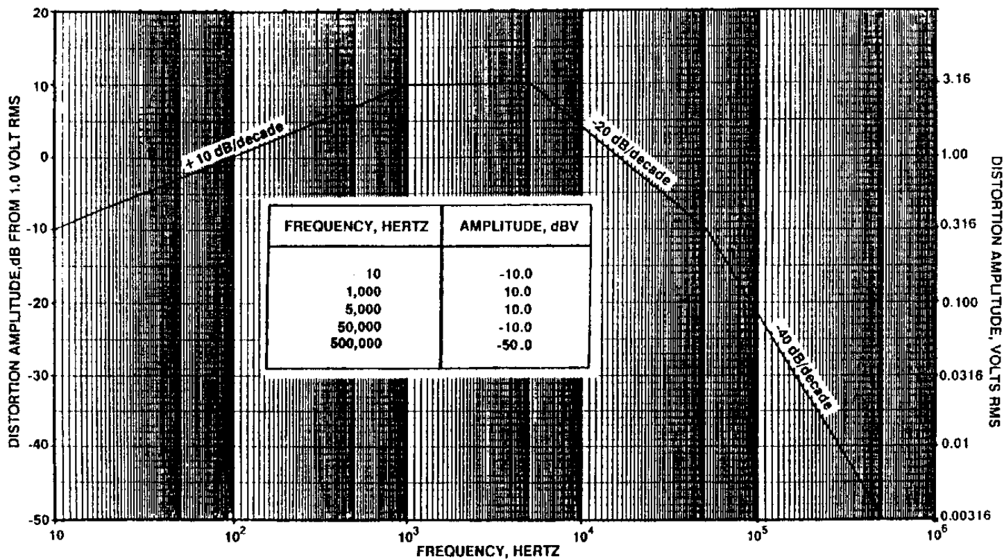
FIGURE 13. Maximum distortion spectrum for 270 volts DC system.
