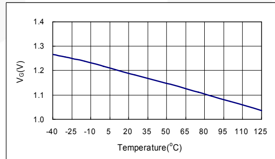
Figure 18. Beginning of Green-Off Mode at V_G
