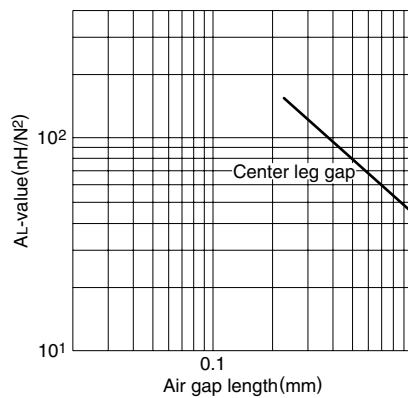
AL-value vs. Air gap length for PC40SEE16 core (Typical)
