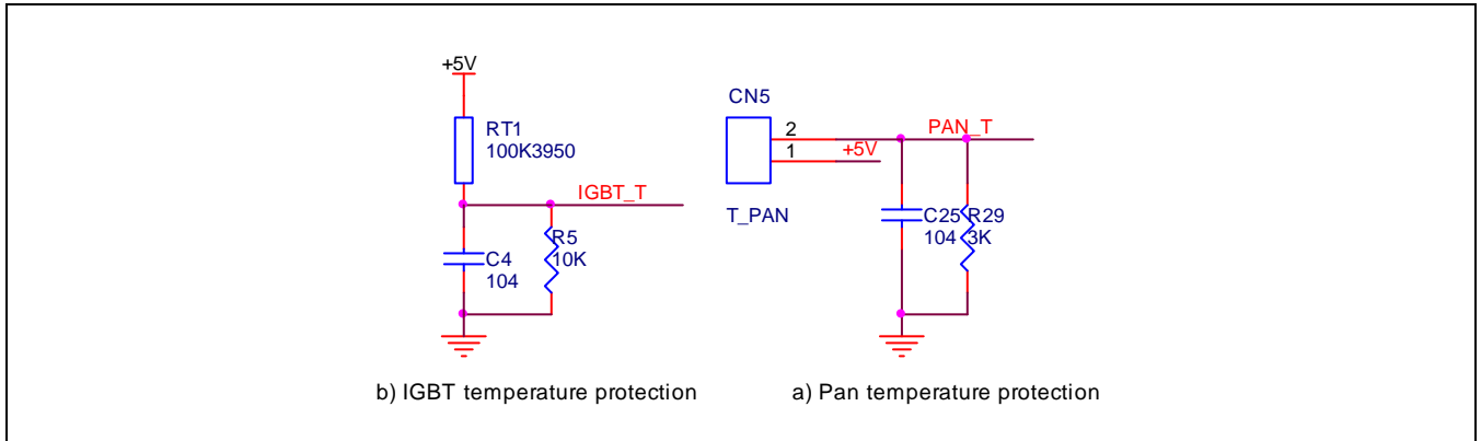
Figure 2-7 Over-Temperature Protection
