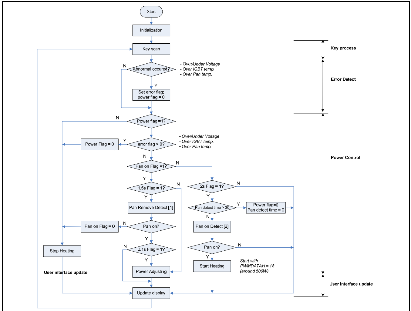
Figure 3-2 Software Diagram
