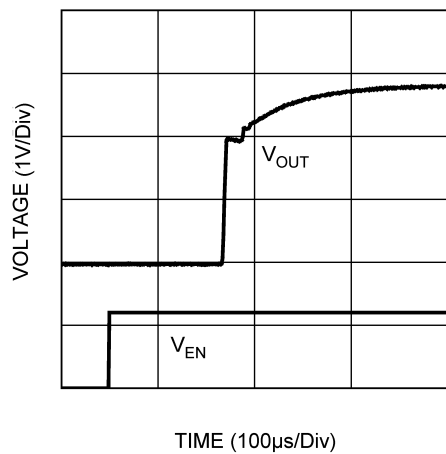
Enable Start-up Time, ( I_L = 1mA , V_{OUT} = 2.8V )
