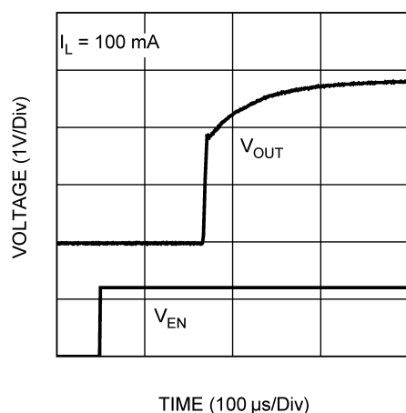
Enable Start-up Time, ( I_L = 100mA , V_{OUT} = 2.8V )
