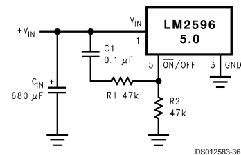
FIGURE 21. Delayed Startup
