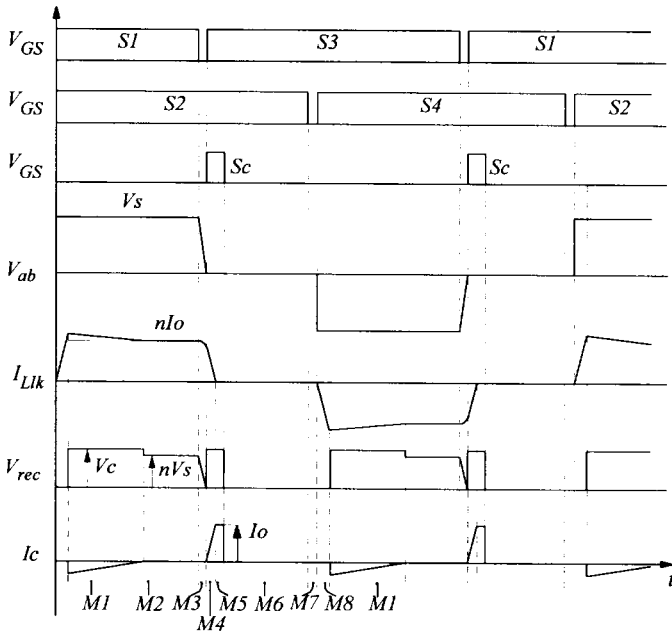
Fig. 3. Operation waveforms.
