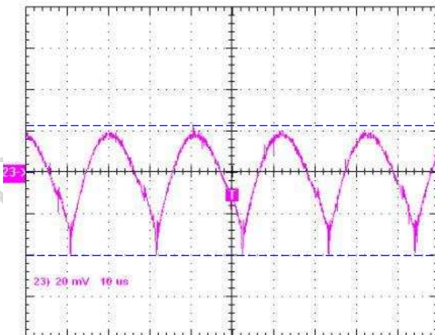
图8 纹波噪声波形, 265Vac, 满载 20mV/div 10us/div
