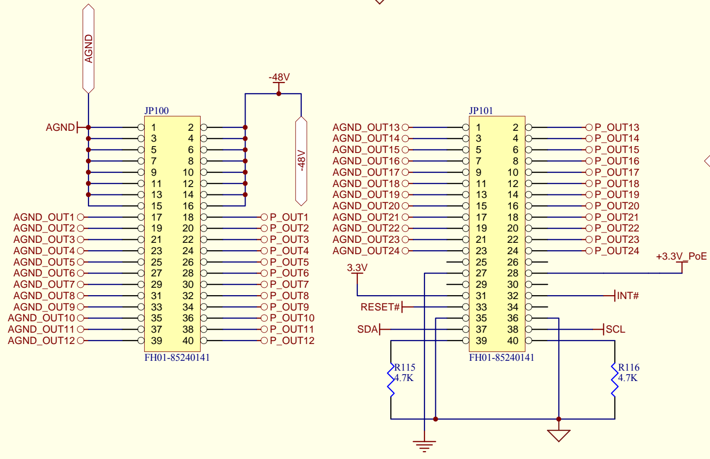
CONNECTOR CIRCUIT
