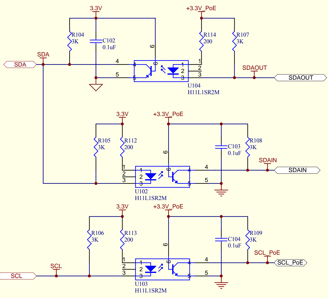
ISOLATION CIRCUIT OF MAX5980 PSE ICM
