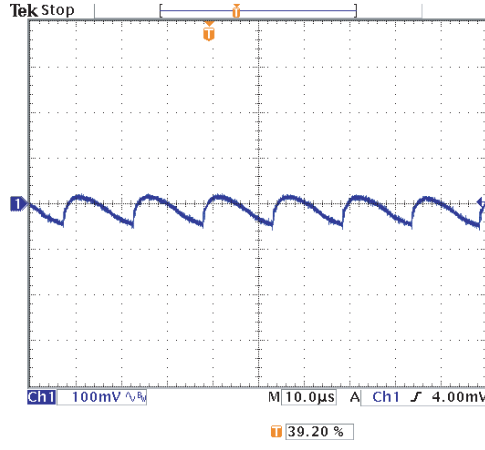
d. Mains input 180 V / 50 Hz (Ch1 = V_{OUT} )
