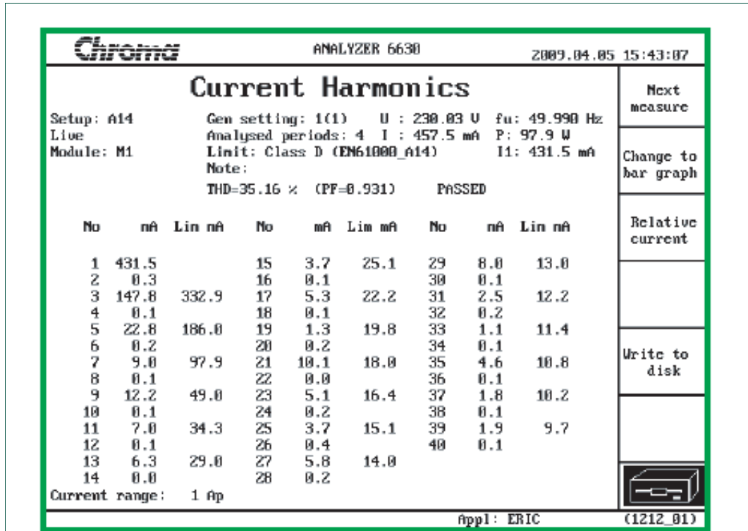
Fig 18. Mains harmonic currents; absolute values
