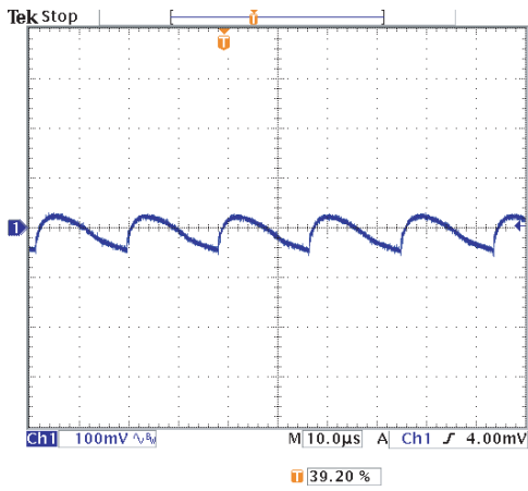
a. Mains input 90 V / 60 Hz (Ch1 = V_{OUT} )
