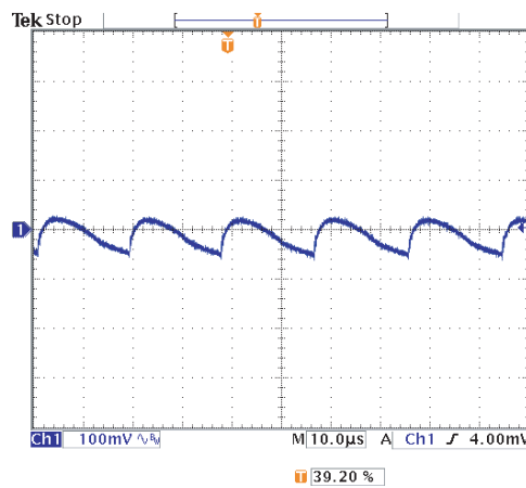
c. Mains input 132 V / 60 Hz (Ch1 = V_{OUT} )
