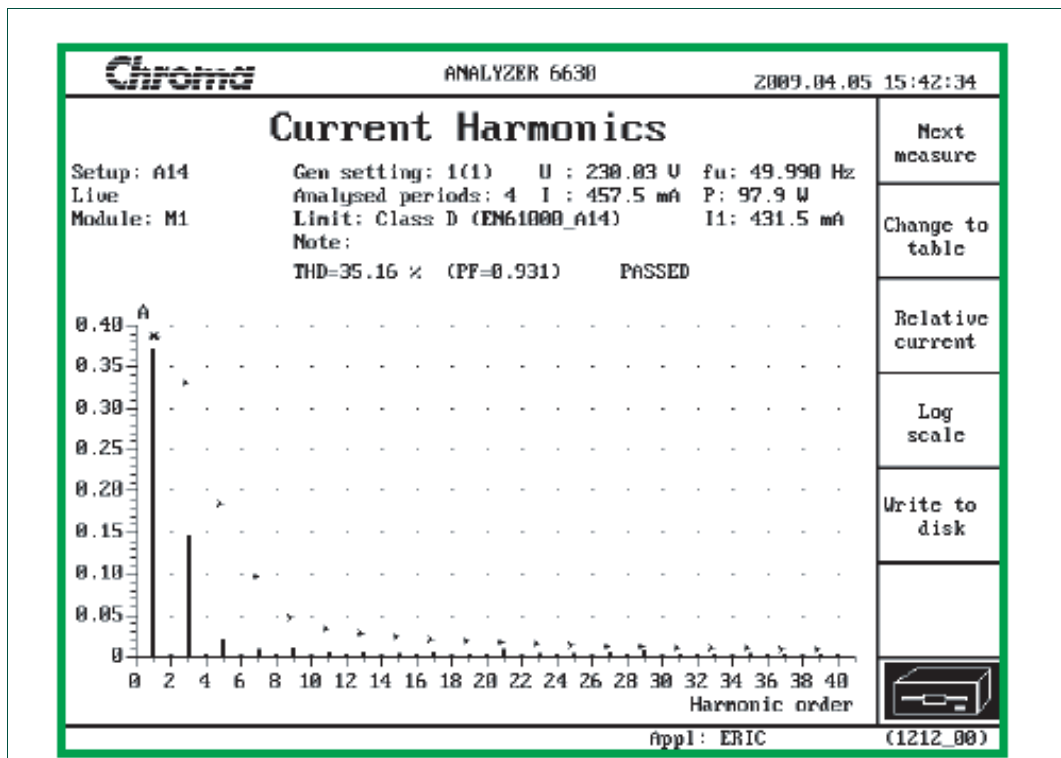
Fig 19. Mains harmonic currents; graphic representation
