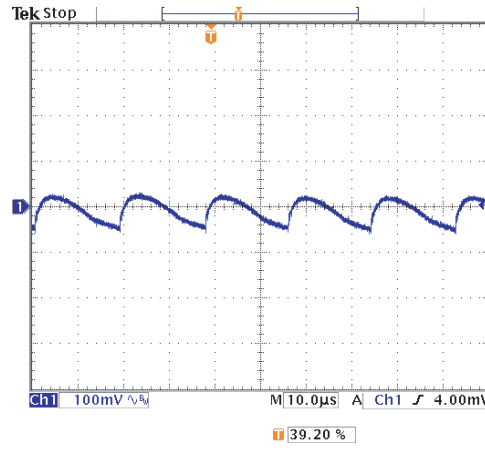
b. Mains input 115 V / 60 Hz (Ch1 = V_{OUT} )
