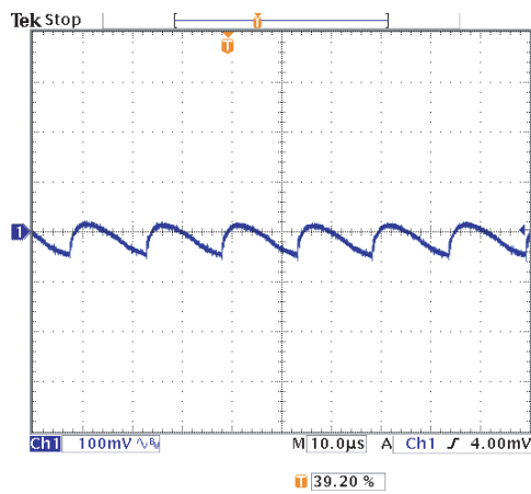
e. Mains input 230 V / 50 Hz (Ch1 = V_{OUT} )
