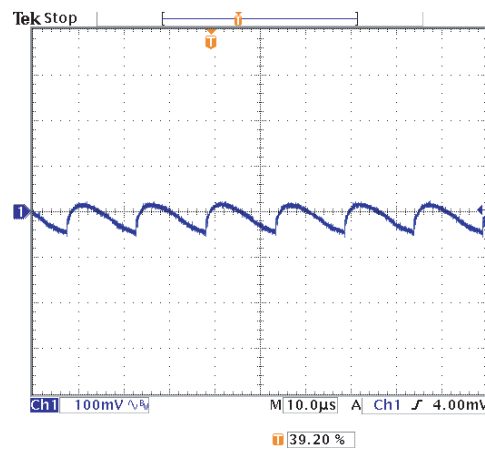
f. Mains input 264 V / 50 Hz (Ch1 = V_{OUT} )
