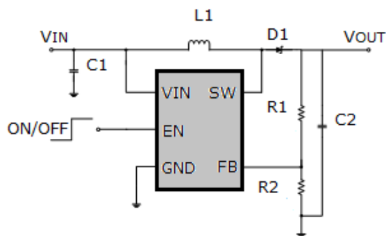
Basic Application Circuit
