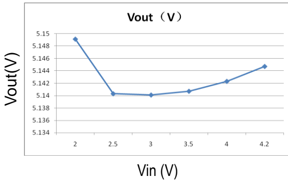
line Regulation
