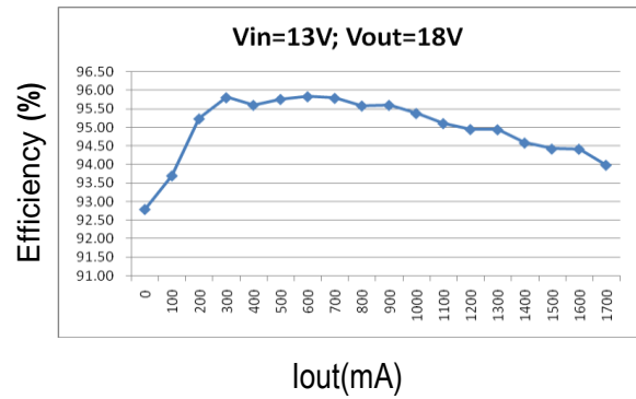
Efficiency Curve
