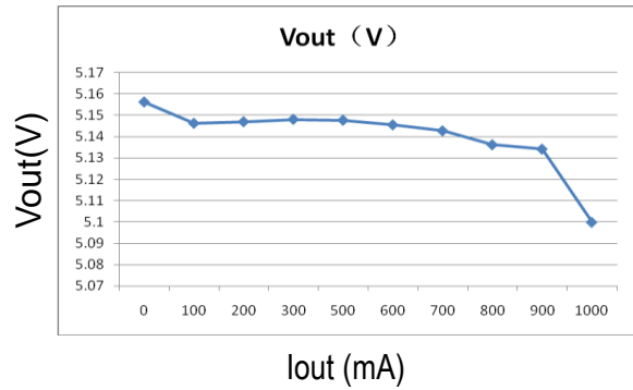
Load regulation
