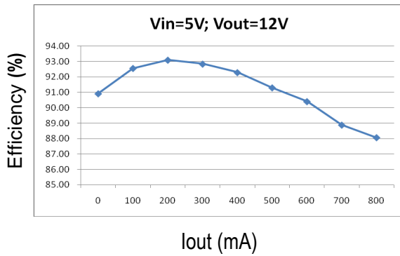
Efficiency Curve
