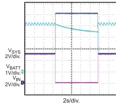
Input Over Voltage Protection, Charge Mode
