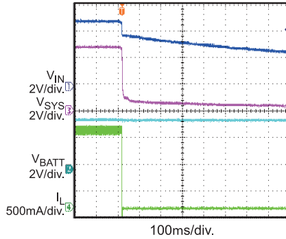
Input Current Limit, Charge Mode
