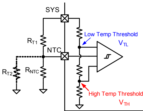
Figure 12: NTC Function Block
