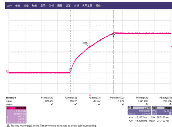
Rise waveform @264Vac input with full load
