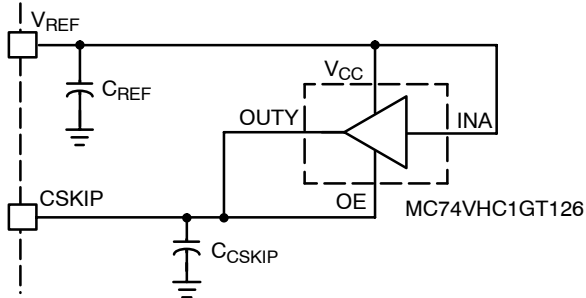
Figure 38. External Latch Implemented using ON Semiconductor's MiniGate™ Buffer
