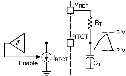
Figure 48. Oscillator Configuration
