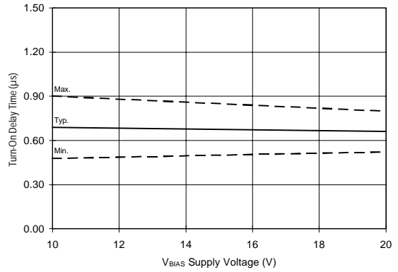
Figure 11B. Turn-On Time vs. Supply Voltage
