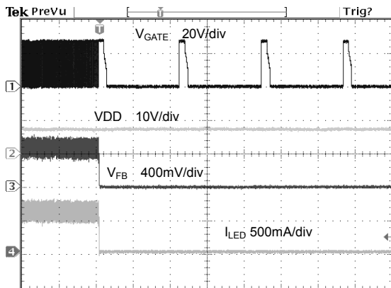
t-2ms/div
