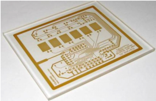
Touch Pads printed on glass
