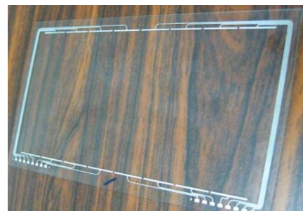
ITO Touch screen on PET film
