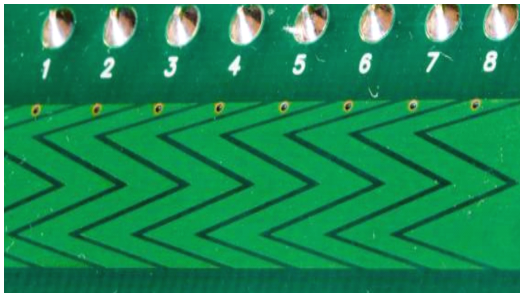
Discrete Slider PCB
