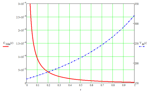
Fig. 19: The relationship between the minimum decoupling capacitance, the DC voltage level, and the voltage ripple
